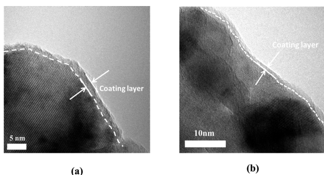
Figure 6. Transmission electron micrographs of (a) TiO 2 ALD-coated (50 ALD cycles) and (b) Al 2 O 3 ALD-coated (15 ALD cycles) nanowire.
